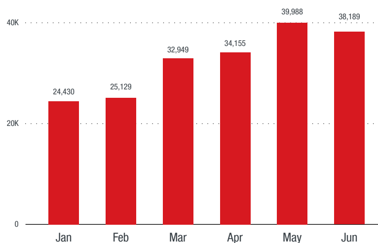
Figure 12. Fileless malware continued to be seen: Fileless events blocked by month in 1H 2018
