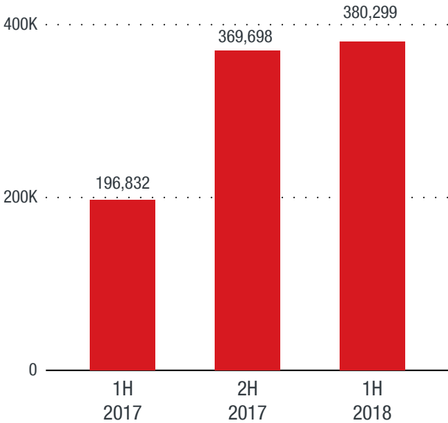
Figure 6. Ransomware detections grew just 3 percent: Half-year comparison of ransomware detections
